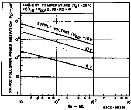
Fig. 13 - Typical source follower power dissipation as a function of R_s .
